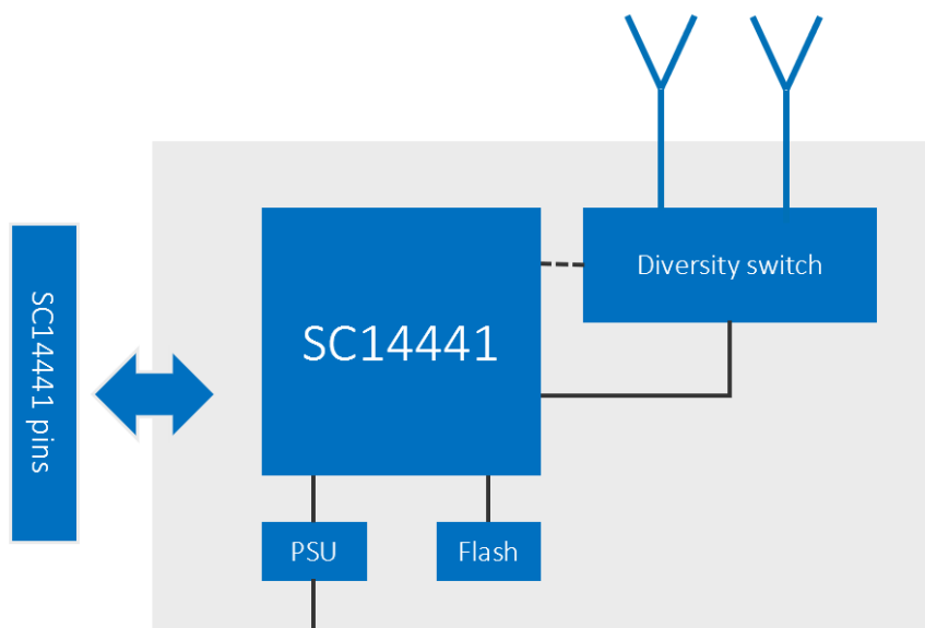
Figure 1: RTX1040 module components
